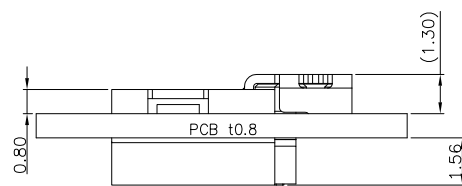
MOUNTING CONDITION (REF.)
