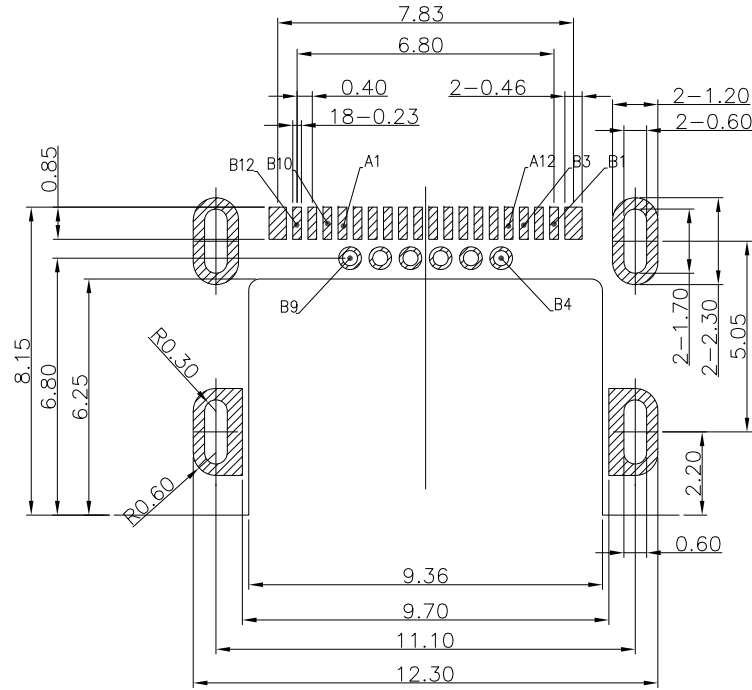
PCB LAYOUT (RECOMMENDED) (Tol:±0.05)
